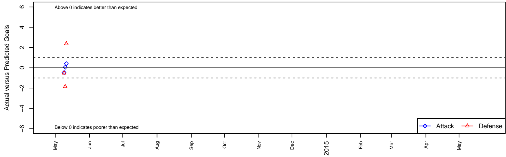
XUnk Johnson B02 Dots are actual minus expected GF (blue circles) and GA (red triangles). Blue line is smoothed change in attack strength. Red is smoothed change in defense strength.
